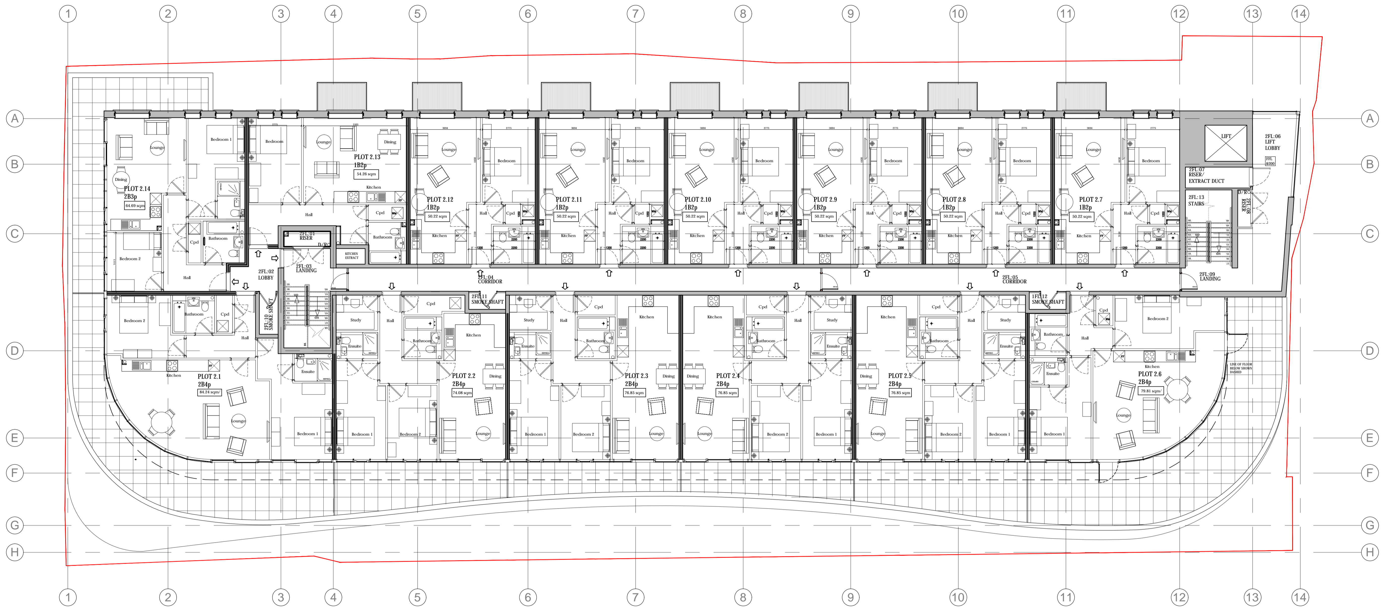
SECOND FLOOR Scale 1:100
